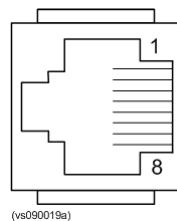
Figure 12 Front view of RJ45 with pin layout
