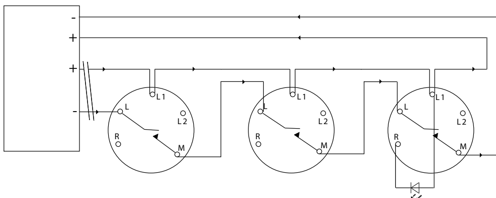
Fig. 7: Typical implementation wiring diagram – 4B-C Continuity Bases
