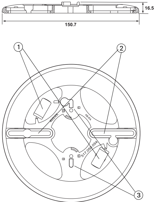
Fig. 12: 4B-6A 4" base 6" adaptor
