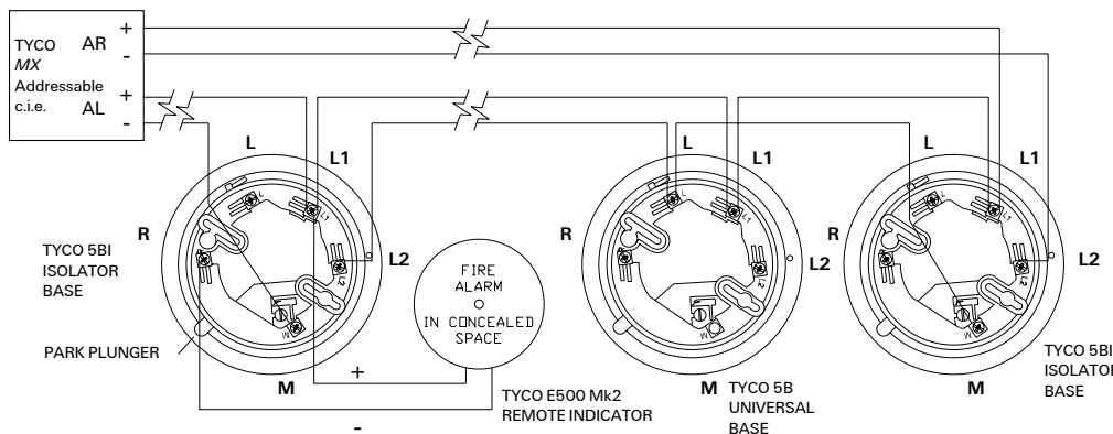
5B Base Wiring—Addressable Systems
