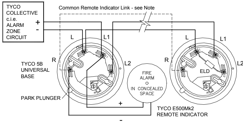
5B Base Wiring—Collective Systems
